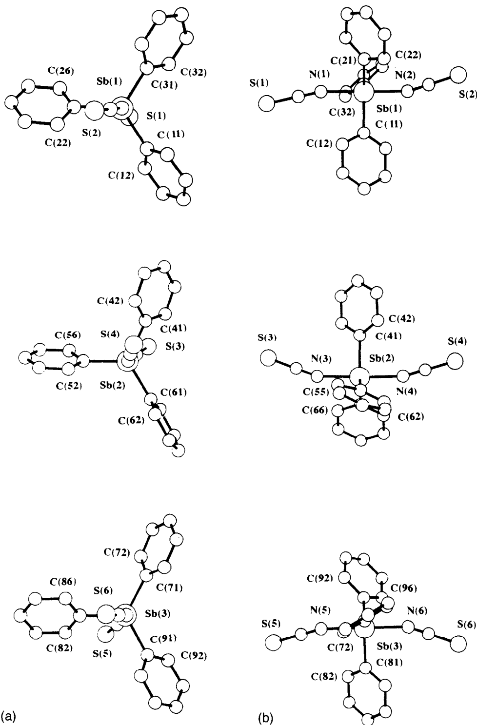
Fig. 1. Structures of the \text{SbPh}_3(\text{NCS})_2 molecules perpendicular to (a) the \text{C}_3\text{Sb} plane and (b) the \text{N-Sb-N} vector.
