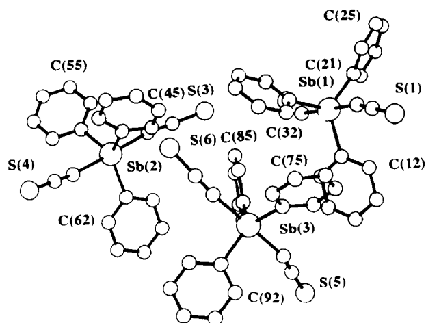
Fig. 2. Relative orientations of the three molecules in the unit cell.
