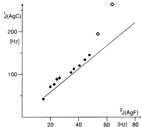
Figure 3. Correlation of ^1J(\text{AgC}) vs ^2J(\text{AgF}) in the mixed \text{CF}_3/\text{CF}_2\text{H} -containing argentates [\text{Ag}(\text{CF}_2\text{H})_n(\text{CF}_3)_{4-n}]^- ( n = 0-4 ) and trans - [\text{Ag}(\text{CF}_2\text{H})_2(\text{CN})_2]^- . Closed diamonds correspond to \text{Ag}(\text{III})-\text{CF}_2\text{H} , closed circles to \text{Ag}(\text{III})-\text{CF}_3 units, and open diamonds to the silver(I) species [\text{Ag}(\text{CF}_2\text{H})_2]^- and [\text{Ag}(\text{CF}_2\text{H})(\text{CN})]^- . The solid line is the fit line for \text{Ag}(\text{III})-\text{CF}_3 derivatives, taken from ref 4.
