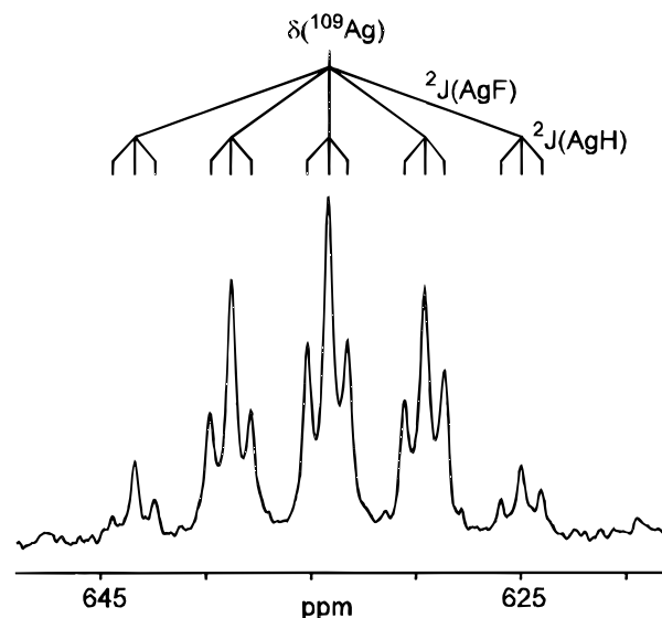
Figure 4. ^{109}\text{Ag} NMR spectrum of the silver(I) species [\text{Ag}(\text{CF}_2\text{H})_2]^- , recorded at -60^\circ\text{C} .
