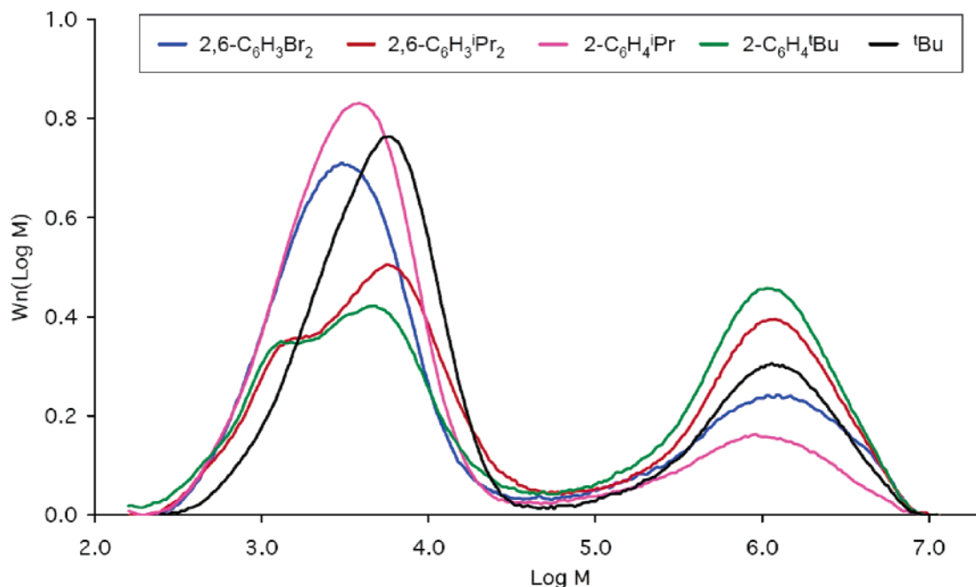
Figure 4. Molecular weight distributions determined by GPC for the polyethylenes produced by MAO-activated \text{Cp}^*\text{Ti}(\text{N}^t\text{Bu})\text{Cl}(\text{py}) ( 1 ) and \text{Cp}^*\text{Ti}(\text{NAr})\text{Cl}(\text{py}) (Ar = 2,6- \text{C}_6\text{H}_3^i\text{Pr}_2 ( 2 ), 2,6- \text{C}_6\text{H}_3\text{Br}_2 ( 3 ), 2- \text{C}_6\text{H}_4^t\text{Bu} ( 4 ), and 2- \text{C}_6\text{H}_4^i\text{Pr} ( 5 )) at 10 \mu\text{mol} precatalyst loadings.
