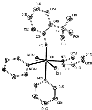
Figure 2. Molecular structure of Ti(N-2-C 6 H 4 CF 3 )Cl 2 (py) 3 (6). Displacement ellipsoids are drawn at the 25% probability level. H atoms are omitted and only one orientation of the disordered 2-C 6 H 4 -CF 3 group is shown. Atoms carrying the suffix “A” are related to their counterparts by the symmetry operator 1–x, y, 1/2–z.
