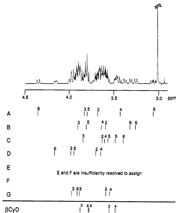
Figure 10. ^1\text{H} -NMR spectrum of DMAB- \beta CyD in the presence of 1-adamantanol in \text{D}_2\text{O} at 25^\circ\text{C} , in the region of cyclodextrin protons, except for C1 protons, and assignments of the protons.
