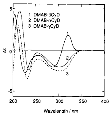
Figure 4. Circular dichroism spectra of DMAB- \alpha CyD, DMAB- \beta CyD, and DMAB- \gamma CyD at 25 °C in an aqueous solution ( 2.5 \times 10^{-5} M). Temperature is 25 °C.
