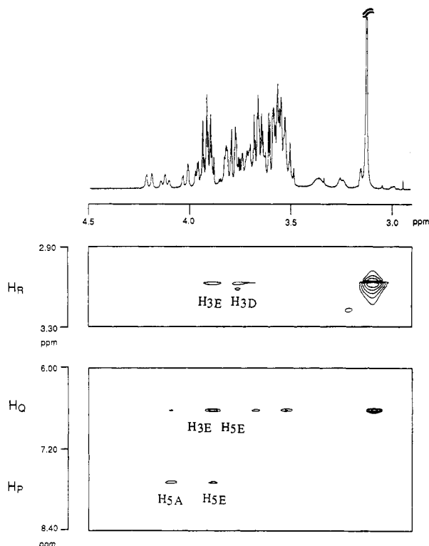
Figure 7. Parts of ROESY spectrum of DMAB- \beta CyD in D 2 O at 25 °C with mixing time of 300 ms, covering the protons of N,N -dimethyl (H R ) and aromatic ring (H P and H Q ). Assignments of cross peaks are also shown.
