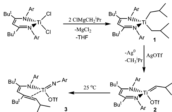
Scheme 1. Synthesis of Complexes 1–3
