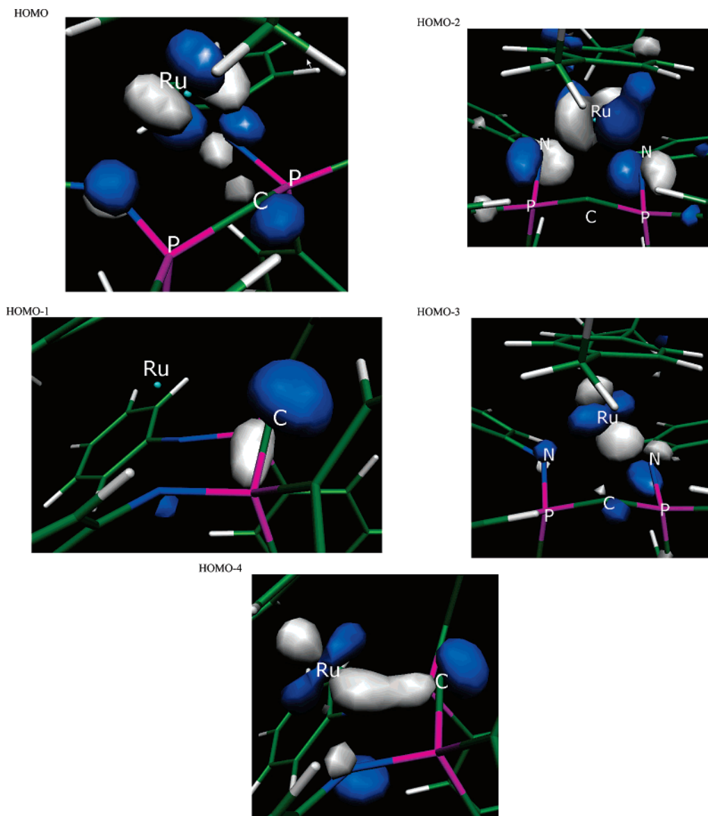
Figure 8. Representation of AO composition of the highest five filled orbitals of (Cym)Ru[ \eta^3 -C(PPh 2 NPh) 2 ] showing the ring carbon "lone pair" (HOMO-1) and three doubly occupied, mainly d orbitals.
