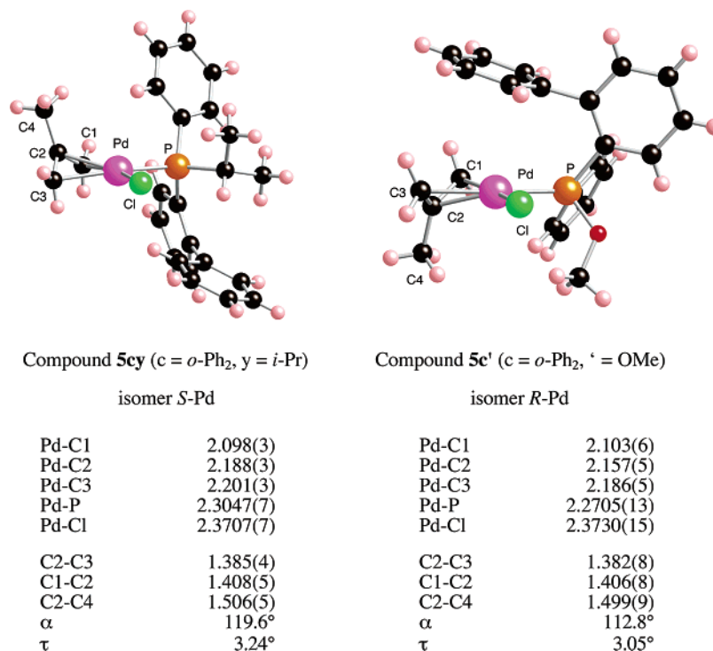
Figure 3. Molecular structures of complexes 5cy and 5c' and selected bond distances (Å) and structural parameters α (angle between planes C1C2C3 and PdClP) and τ (dihedral angle PC1C3C1). 66
