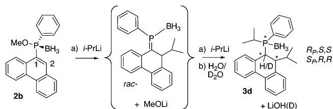
Scheme 2. Proposed Formation of 3d
