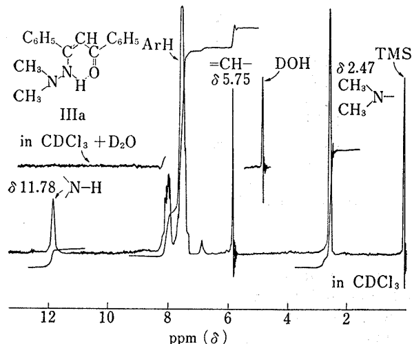
Fig. 1. NMR Spectra of IIIa In CDCl 3
