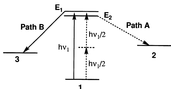
Figure 3. Schematic representation of selective photoreactions via NRTP.
