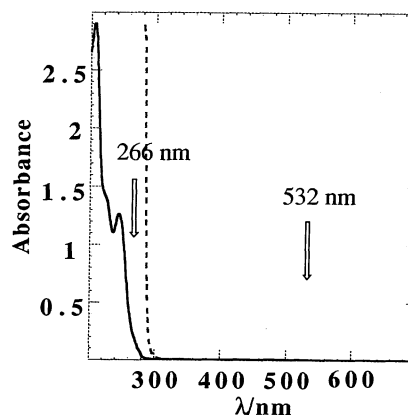
Figure 1. Absorption spectra of 1 in hexane: c = 7.49 \times 10^{-5} M (—); c = 7.31 \times 10^{-3} M (-----). Arrows denotes wavelengths of laser lights, 266 and 532 nm, for excitation.
