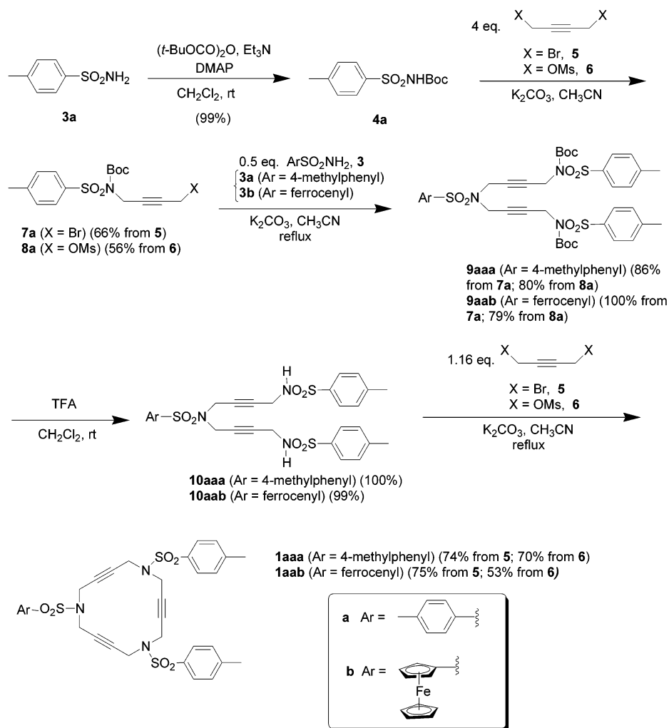
Scheme 1. Synthesis of Macrocycles 1aaa and 1aab
