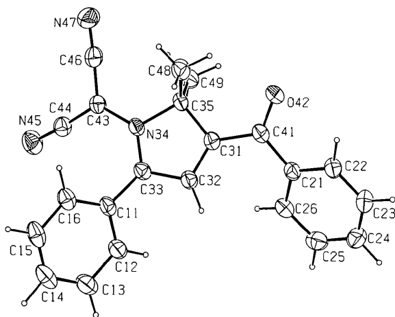
Fig. 2. The molecular structure of compound (V) showing the labelling of the non-H atoms. Displacement ellipsoids are shown at 50% probability levels and H atoms are drawn as small circles of arbitrary radii.
