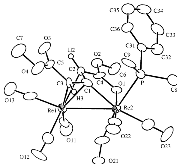
Figure 3. ORTEP diagram of fac -Re 2 (CO) 6 (PMe 2 Ph)[ \mu - \eta^3 - \eta^1 -MeO 2 C(H)CCC(H)CO 2 Me], 4 , showing 40% probability thermal ellipsoids. Selected interatomic distances (Å) and angles (deg): Re(1)–Re(2) = 3.0069(9), Re(1)–C(1) = 2.14(1), Re(1)–C(2) = 2.31(1), Re(1)–C(3) = 2.39(1), Re(2)–C(1) = 2.15(2), Re(2)–O(1) = 2.20(1), Re(2)–P = 2.474(4), C(1)–C(2) = 1.47(2), C(1)–C(3) = 1.40(2), C(2)–C(4) = 1.44(2), C(4)–O(1) = 1.23(2), C(5)–O(3) = 1.18(2); C(2)–C(1)–C(3) = 119(2), C(1)–Re(2)–P = 80.9(4), Re(1)–Re(2)–P = 126.0(1).
