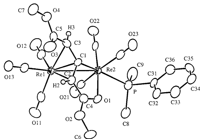
Figure 2. ORTEP diagram of mer -Re 2 (CO) 6 (PMe 2 Ph)[ \mu - \eta^3 - \eta^1 -MeO 2 C(H)CCC(H)CO 2 Me], 3 , showing 40% probability thermal ellipsoids. Selected interatomic distances (Å) and angles (deg): Re(1)–Re(2) = 2.9727(3), Re(1)–C(1) = 2.089(8), Re(1)–C(2) = 2.331(8), Re(1)–C(3) = 2.358(8), Re(2)–C(1) = 2.156(7), Re(2)–O(1) = 2.192(6), Re(2)–P = 2.443(2), C(1)–C(2) = 1.42(1), C(1)–C(3) = 1.41(1), C(2)–C(4) = 1.43(1), C(4)–O(1) = 1.25(1), C(5)–O(3) = 1.21(1); C(2)–C(1)–C(3) = 121.6(8), C(1)–Re(2)–P = 158.9(2), Re(1)–Re(2)–P = 148.15(6).
