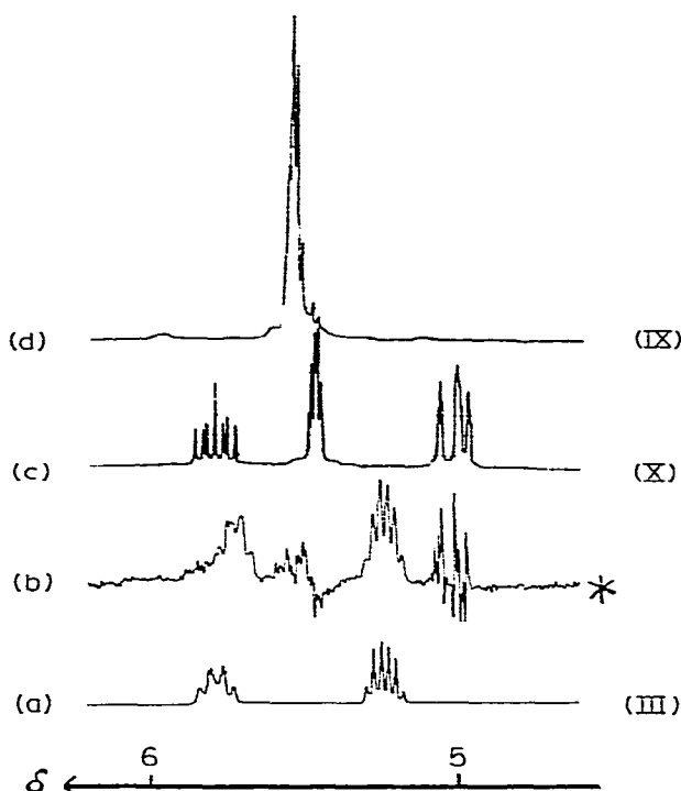
Fig. 3. Olefin part in the 270 MHz ^1\text{H} NMR spectra: (a) III at 25°C, (b) III at 100°C during the thermal decomposition, (c) X ( trans ) at 25°C, and (d) IX ( trans,trans ) at 25°C.
