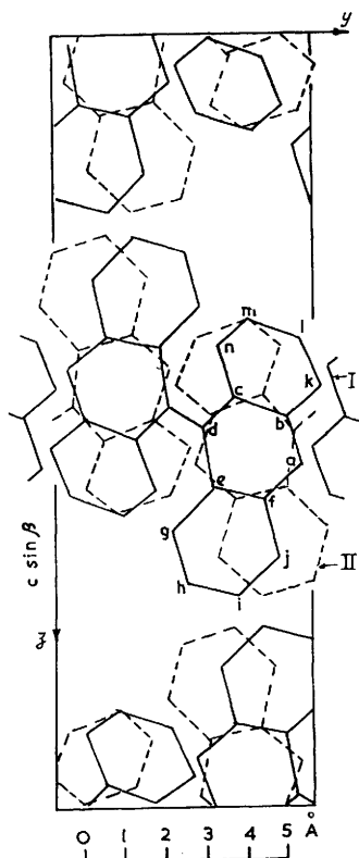
FIG. 5(a). \alpha -Bixanthenylidene in x -projection.
