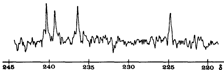
Fig. 2. Section of the 100.613 MHz ^{13}\text{C} NMR spectrum of [(\text{C}_5\text{Me}_5)\text{Mo}(\text{CO})_2]_2(\text{PhC}\equiv\text{CH}) in the metal carbonyl region.
