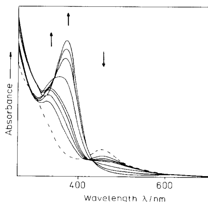
Fig. 3. UV-Vis spectral changes upon irradiation of 10^{-2} M IV and 0.3 M \text{P(OMe)}_3 in THF in a 0.2 mm IR cell. --- before, — after irradiation at 457.5 nm.
