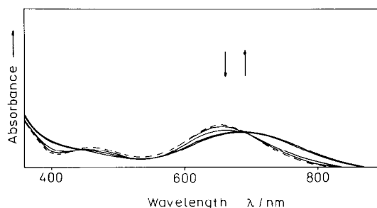
Fig. 2. UV-Vis spectral changes upon irradiation of 10^{-2} M I and 0.3 M \text{P}^t\text{Bu}_3 in THF in a 0.2 mm IR cell. --- before, — after irradiation at 457.5 nm.
