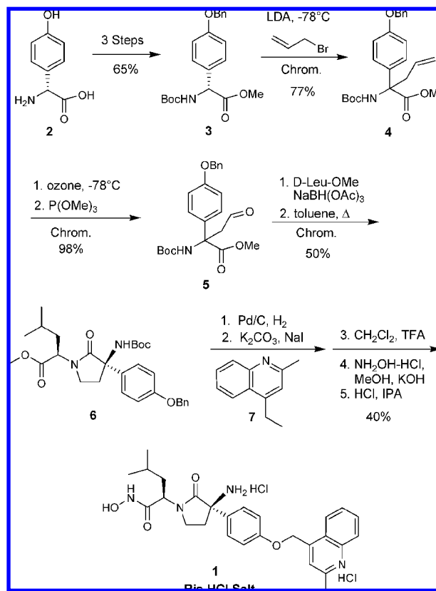
Scheme 1. Original synthesis of BMS-561392
