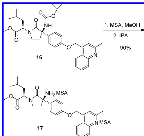
Scheme 7. Boc cleavage to form final intermediate 17
