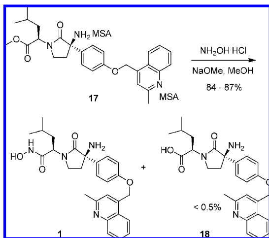
Scheme 8. Hydroxamate formation to give target 1
