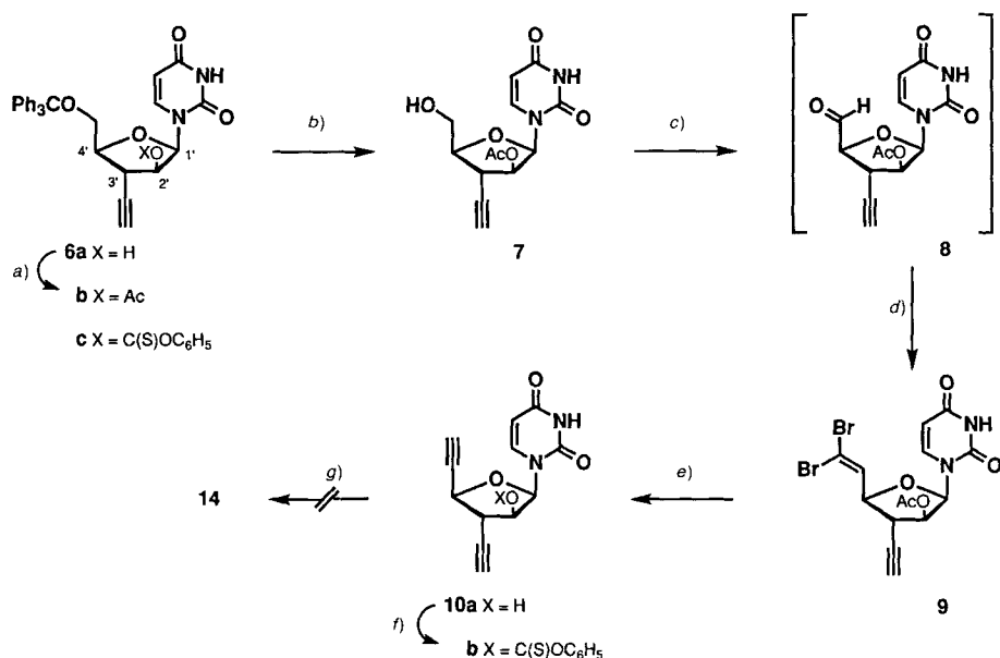
Scheme 2. Attempted Synthesis of 3',4'-Diethynyl-2',3',5'-trideoxy-5'-noruridine ( 14 )
