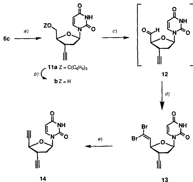
Scheme 3. Synthesis of 3',4'-Diethynyl-2',3',5'-trideoxy-5'-noruridine ( 14 )
