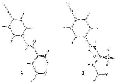
Figure 1. Comparative arrays of (A) L-aspartyl- p -cyanoanilide ( 3 ) and (B) trifluoroacetyl-L-aspartyl- p -cyanoanilide ( 2 ). The orientation and location of the carboxylate are fixed. Hydrogen bonds are indicated by dashed lines.
