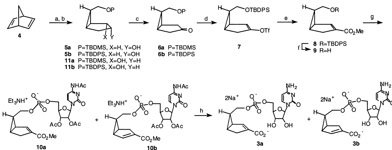
Scheme 1. Reagents and conditions: (a) (i) m -CPBA; (ii) NaBH 4 ; (iii) TBDMSCl or TBDPSCl, imidazole. (b) (i) BH 3 ·SMe 2 ; (ii) H 2 O 2 , NaOH, 90–95%. (c) CrO 3 , pyridine, 78% for 6a ; 86% for 6b . (d) Tf 2 O, 2,6-di- tert -butyl-4-methylpyridine, 69%. (e) Pd(OAc) 2 , PPh 3 , Et 3 N, MeOH, CO, DMF, rt, 80%. (f) TBAF, THF, 85%. (g) (i) Cytidine-2',3'-di- O -acetyl-4- N -acetyl-5'-( N,N -diisopropyl-2-cyanoethyl)-phosphoramidite, 1 H -tetrazole, CH 2 Cl 2 ; (ii) t -BuOOH; (iii) Et 3 N, CH 2 Cl 2 , 51% for three steps. (h) (i) NaOMe, MeOH–H 2 O; (ii) HPLC (MonoQ, NH 4 HCO 3 –MeOH–H 2 O); (iii) desalting with Amberlite IR-120, 30%.
