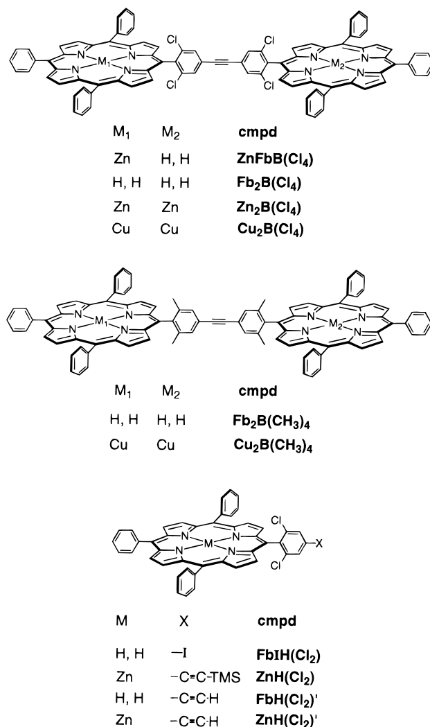
Chart 2. Structures of Dimeric Arrays and Porphyrin Building Blocks
