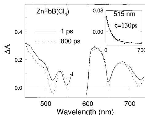
Figure 2. Transient difference spectra acquired following excitation of ZnFbB(Cl 4 ) in toluene at room temperature with a 0.2-ps flash at 582 nm. The spectra for the array was acquired with time delays of 1 ps (solid traces) or 800 ps (dashed traces). Note that the data in the red region were acquired with a sample concentration \sim 10 -fold greater than that used for the blue region. Consequently, a quantitative comparison of the absorption changes in the two regions should not be made. The inset shows a representative kinetic trace at 515 nm with a fit to a dual exponential which takes into account both the fast decay of Zn* and the slow decay of Fb*. The Fb* lifetime was fixed at the value of 4.6 ns obtained from the fluorescence lifetime measurements (Table 1).
