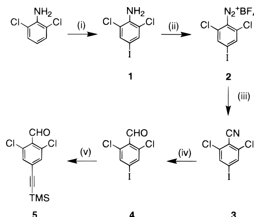
Scheme 1. Aldehyde Precursors for Preparing the Porphyrins a
