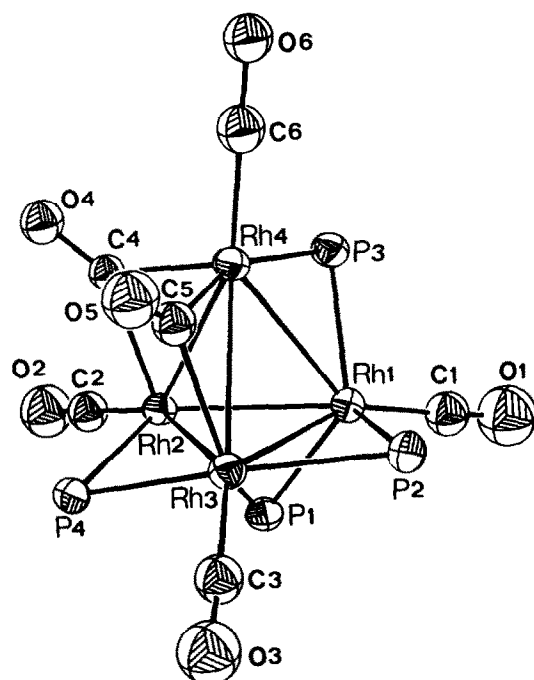
Fig. 1. A perspective view of the stereochemistry of [\text{Rh}_4(\mu\text{-PPh}_2)_4(\mu\text{-CO})_2(\text{CO})_4] , 1a , showing the atom labelling scheme and thermal ellipsoids at the 30% probability level.
