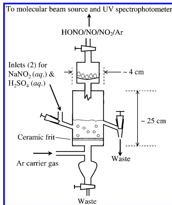
Figure 2. Schematic diagram of the HONO generator, which was based on the designs of Ning and Pfab (ref 31) and Marshall and Midgeley (ref 32) and has incorporated our modifications.
