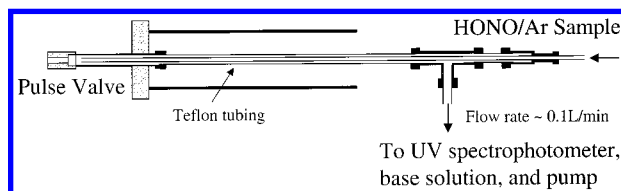
Figure 3. Schematic diagram of the flow system of the HONO sample into the molecular beam.
