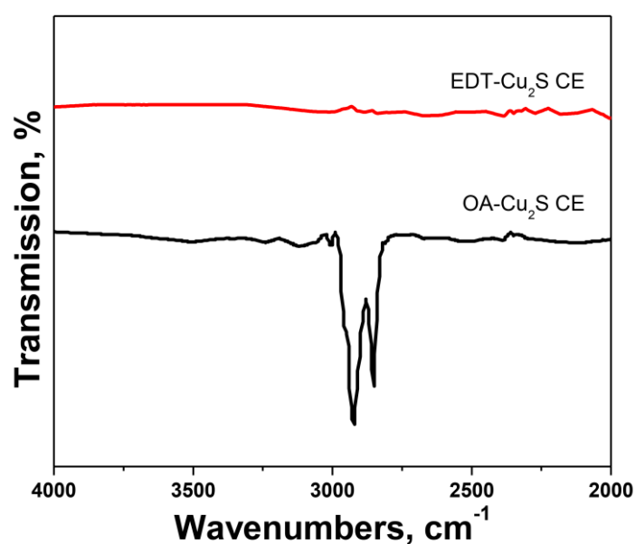
Figure 4. FT-IR spectra of OA-, EDT-Cu 2 S NCs annealed at 80 °C for 30 min
