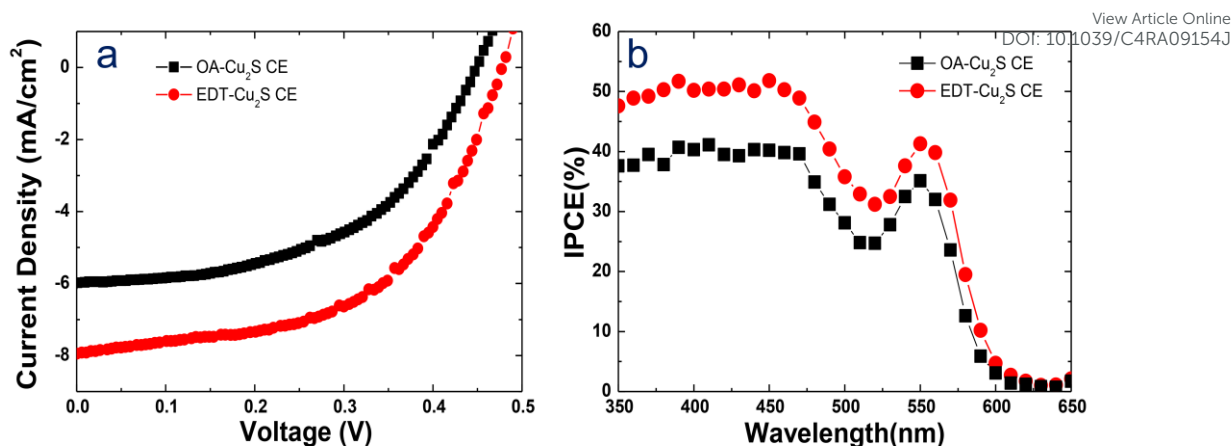
Figure 3. (a) Photocurrent-voltage characteristics of CdSe QDSSCs with Cu 2 S CE (with EDT, OA-Cu 2 S), measured under AM 1.5 illumination (100 mWcm -2 ); (b) IPCE spectra of the CdSe QDSSCs using Cu 2 S CE (with EDT, OA-Cu 2 S).
