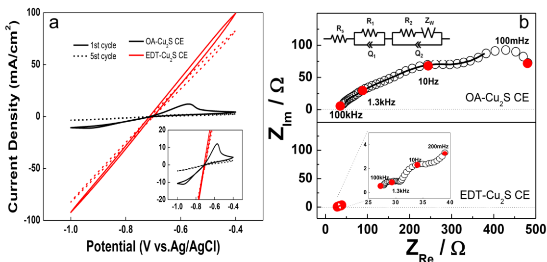
Figure 5. (a) Cyclic voltammograms (CVs) of OA-, EDT-Cu 2 S NCs films measured in polysulfide (1M Na 2 S/1M S) solution, at a scan rate of 50 mV s -1 . (b) Nyquist plots of OA-, EDT-Cu 2 S films measured at the equilibrium potential of the polysulfide. The experimental spectra are denoted with circles, and the best-fitted results using the equivalent circuit with solid lines.
