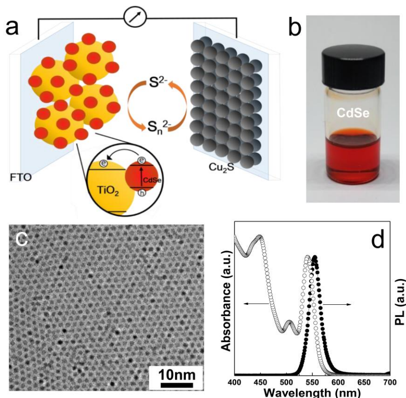
Figure 1. (a) Schematic diagram of QDSSC, (b) Photographic image of colloidal CdSe NCs dispersed in toluene, (c) TEM image of as-synthesized CdSe NCs, (d) Absorption and photoluminescence spectrum of colloidal CdSe NCs
