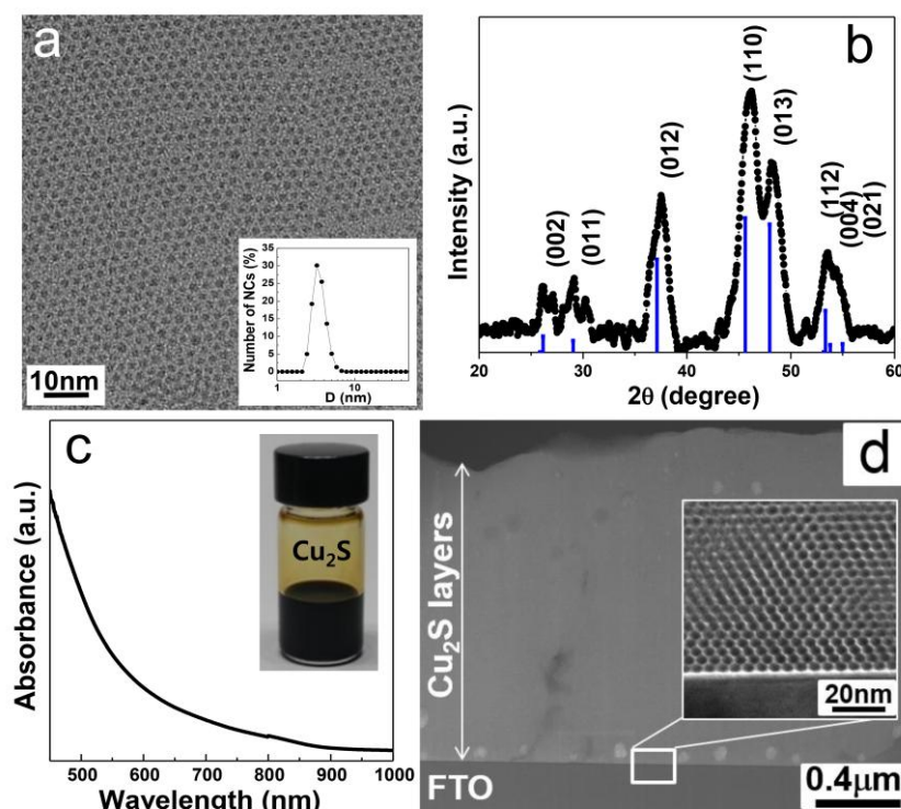
Figure 2. (a) TEM image of as-synthesized Cu 2 S NCs. The inset shows the average size distribution of Cu 2 S NCs based on dynamic light scattering (DLS). (b) XRD patterns of Cu 2 S films: the blue line is JCPDS 90-020-0988 (Hexagonal, P63/mmc space group). (c) Absorption spectra of the Cu 2 S NCs. The inset shows an image of colloidal Cu 2 S NCs dispersed in toluene. (d) Cross-section TEM image of closed-packed EDT-Cu 2 S CE assembled on the FTO substrate.
