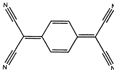
Fig. 7. Valence model representation of TCNQ.
