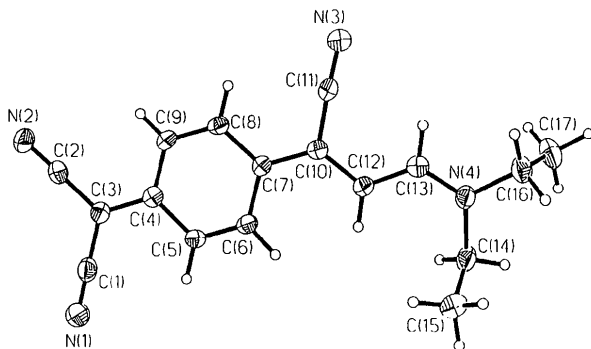
Fig. 4. A 50% probability thermal ellipsoid plot of structure (III).
