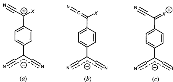
Fig. 8. Valence model resonances of monosubstituted TCNQ derivatives.
