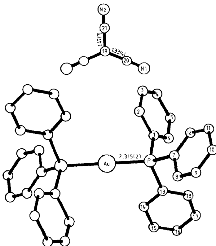
Fig. 1. The structures of the cation and the anion.
