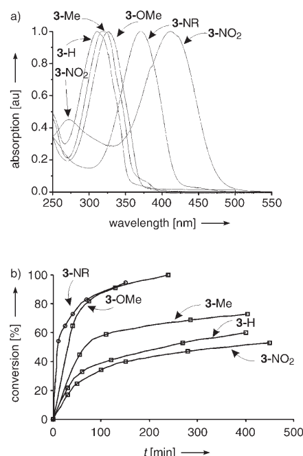
Figure 2. a) UV/Vis spectra for 3b , c–f recorded in \text{CH}_2\text{Cl}_2 . b) Conversion profiles in the Pd-catalyzed AAA between 4a and 5a for variously substituted DATs.
