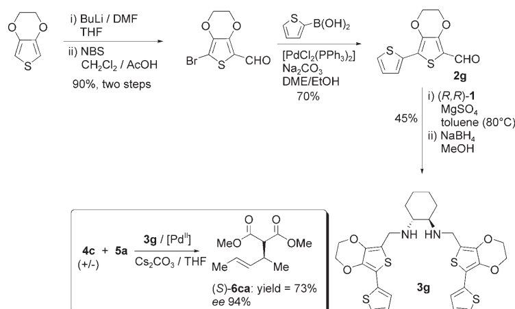
Scheme 3. Synthesis of AEDOT-T ( 3g ) and its application in the AAA between 4c and 5a : i) EDOT (1 equiv), n BuLi (2.5 M, 1 equiv), −78 °C → 0 °C (over 20 min) → −78 °C, then DMF (1.9 equiv), RT, 1 h; ii) EDOT-CHO (1 equiv), N -bromosuccinimide (1 equiv), CH 2 Cl 2 /AcOH 1:1, 0 °C, 2 h (in the dark) 95 %. 2g : [PdCl 2 (PPh 3 ) 2 ] (3 mol %), Na 2 CO 3 (5 equiv), DME/EtOH 1:1, 50 °C, 16 h. 3g : i) ( R,R )- 1 (1.0 equiv), 2g (2.0 equiv), MgSO 4 (10.0 equiv), toluene, 80 °C, 48 h; ii) NaBH 4 (5.0 equiv), MeOH, RT, 16 h, 45 % (two steps).
