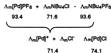
Scheme 2. All values \Lambda_m in \text{S cm}^2 \text{ mol}^{-1} .
