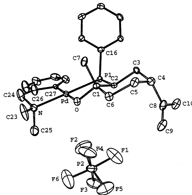
Fig. 2. ORTEP view of the molecular structure of [(\text{dmbs})\text{Pd}(\text{P},\text{OH})]\text{PF}_6 ( 3 ). The second phenyl substituent at P is not shown for clarity. Thermal ellipsoids are drawn at the 30% probability level.
