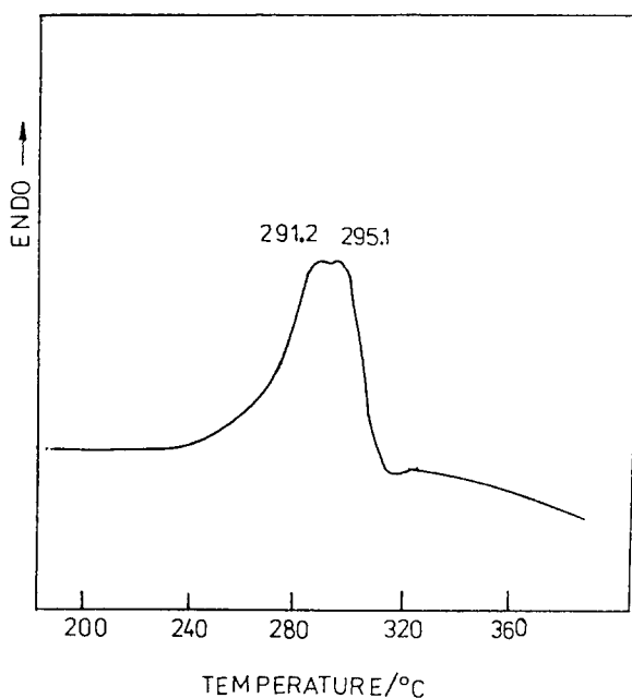
Fig. 4. DSC curve of K_2Mg(IO_3)_4 \cdot 2H_2O .
