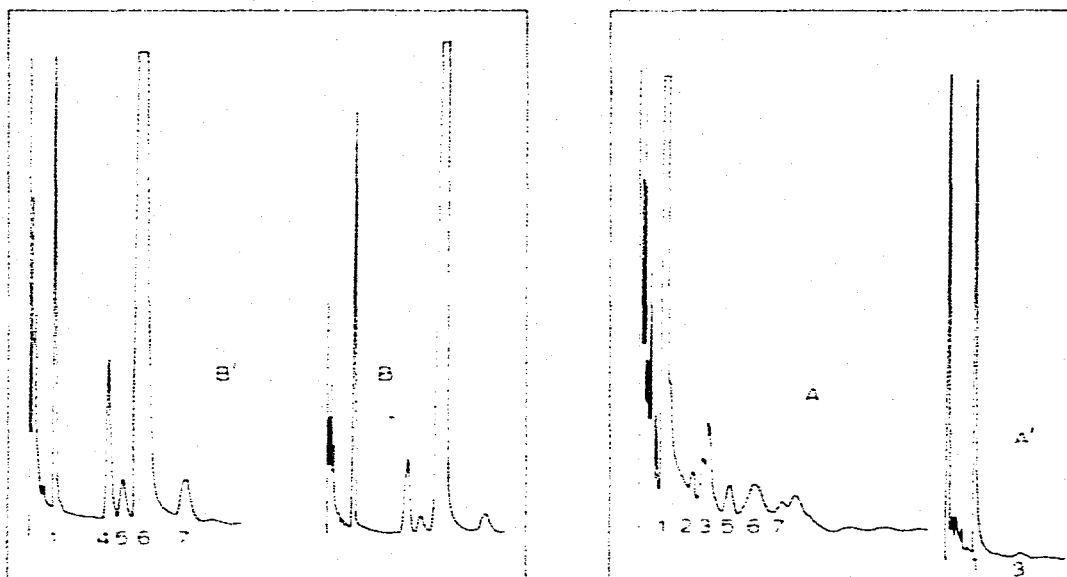
Fig. 1. A. System I, (\text{Ph}_3\text{P})_3\text{CoCl} + \text{CH}_3\text{MgCl} + \text{PhC}\equiv\text{CPh} , under argon. A', lower detector sensitivity.
