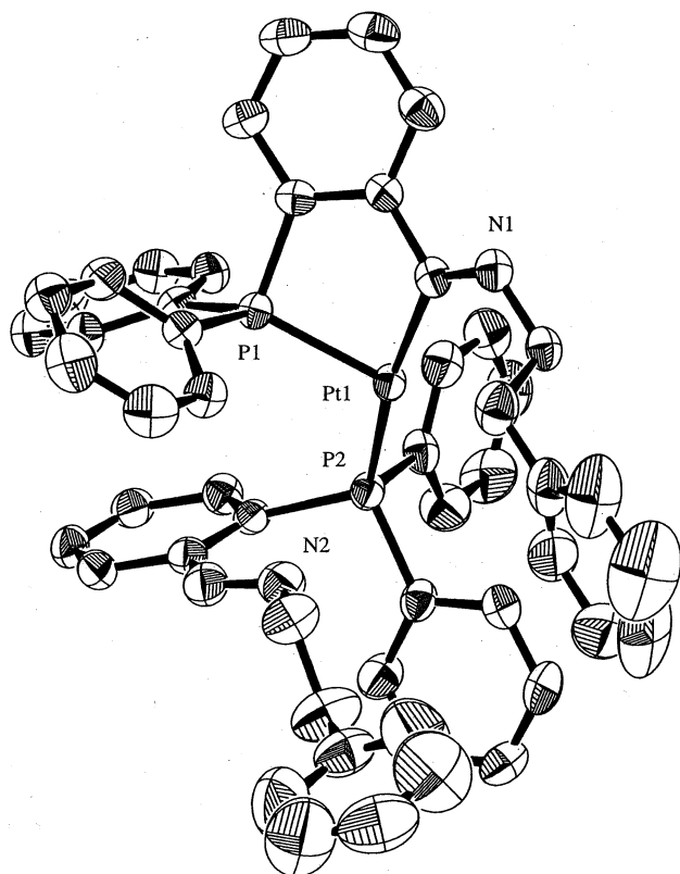
Figure 1. ORTEP diagram of 3 .
