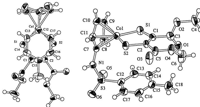
Fig. 3. ORTEP drawing of [(\text{Cp}-\text{NH}-\text{SO}_2-\text{C}_6\text{H}_4-\text{CH}_3)\text{Co}(\text{S}_2\text{C}_2(\text{COOMe})_2)] ( 7 ). Selected bond lengths ( \text{\AA} ): Co–S1 2.112(3), Co–S2 2.102(3), S1–C1 1.697(10), S2–C2 1.726(9), C1–C2 1.35(1), N1–C7 1.38(1). Selected bond angles ( ^\circ ): S1–Co–S2 91.8(1), Co–S1–C1 105.1(3), Co–S2–C2 104.7(3), S1–C1–C2 119.6(7), S2–C2–C1 118.9(7), S3–N1–C7 126.5(7), C7–N1–H11 116.8(8), S3–N1–H11 116.6(6). Plane angles ( ^\circ ): Cp ring/dithiolene ring 88.84, Cp ring/phenyl ring 89.4, dithiolene ring/phenyl ring 12.35.
