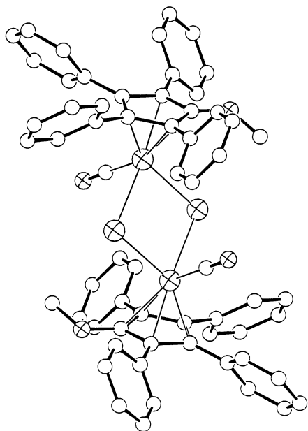
Fig. 5. Molecular structure and selected crystallographic data for 8 . Bond lengths in Å: Ru1–I 2.7271(5); Ru1–I* 2.7338(4); Ru1–C2 1.869(4); C2–O3 1.144(5); C6–O11 1.333(4); Ring C–C (av.) 1.450 \pm 0.020 .
