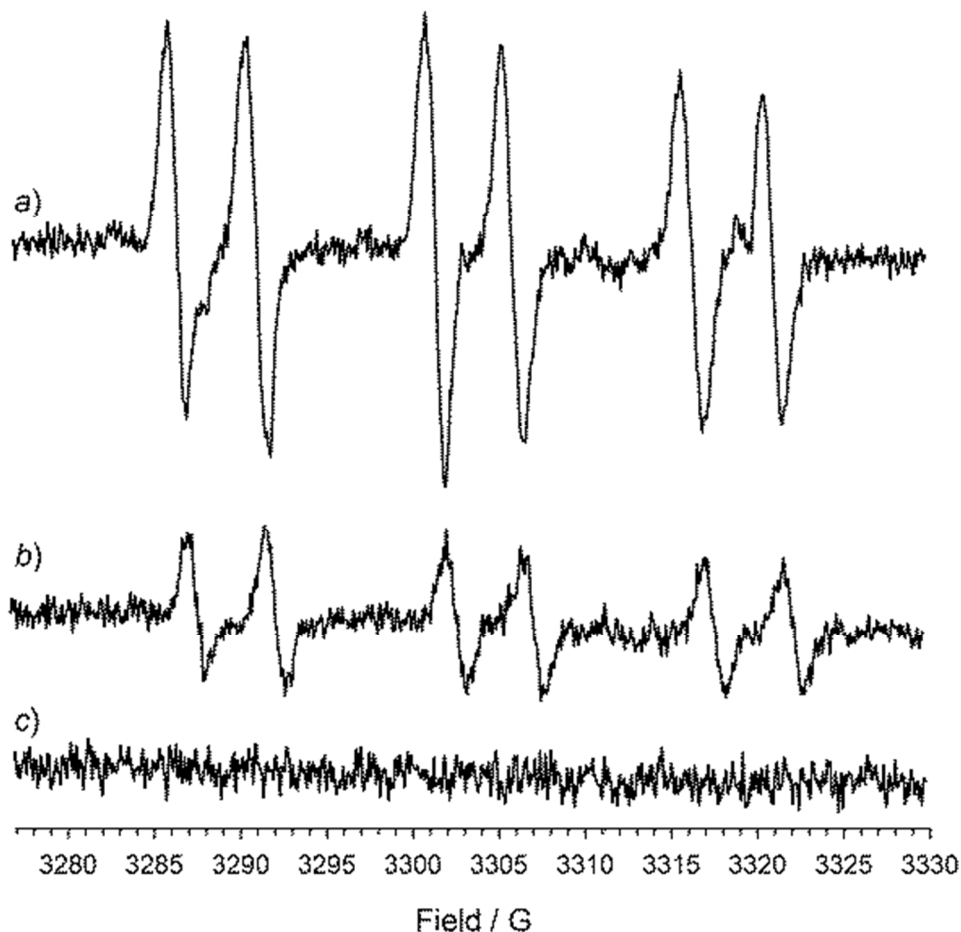
EPR spectra of spin adduct 17 generated in DMF in the presence of dimethyl bromomalonate 2a (0.5 M) and PBN (0.1 M) as the spin trap at room temperature. Reaction conditions: a) [\text{Fe}(\text{bpy})_3]\text{Br}_2 (10 mol%), irradiation with UV-visible light ( \lambda > 320 nm); b) [\text{Fe}(\text{bpy})_3]\text{Br}_2 (10 mol%), irradiation with visible light ( \lambda > 420 nm); c) [\text{Fe}(\text{bpy})_3]\text{Br}_2 (10 mol%) no irradiation. 163x153mm (96 x 96 DPI)
