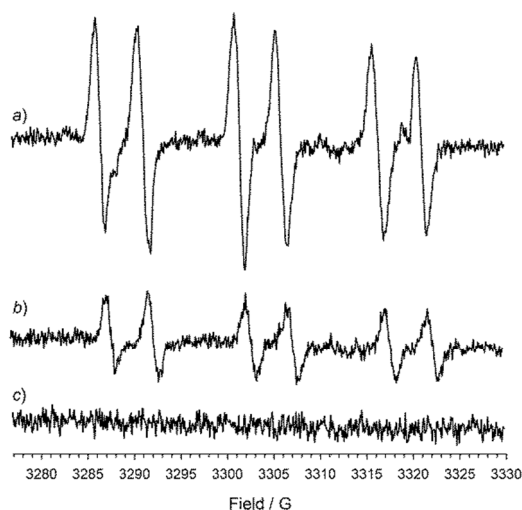
FIGURE 2. EPR spectra of spin adduct 17 generated in DMF in the presence of dimethyl bromomalonate 2a (0.5 M) and PBN (0.1 M) as the spin trap at room temperature. Reaction conditions: a) [\text{Fe}(\text{bpy})_3]\text{Br}_2 (10 mol%), irradiation with UV-visible light ( \lambda > 320 nm); b) [\text{Fe}(\text{bpy})_3]\text{Br}_2 (10 mol%), irradiation with visible light ( \lambda > 420 nm); c) [\text{Fe}(\text{bpy})_3]\text{Br}_2 (10 mol%) no irradiation.
