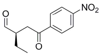
75 76 11 , 55%, 81% ee
