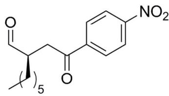
83 84 12 , 53%, 87% ee
