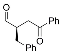
67 68 10 , 40%, 92% ee
