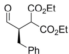
30 31 5 , 78%, 92% ee
