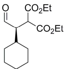
52 53 8 , 75%, 97% ee
