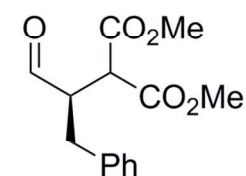
22 23 4 , 83%, 92% ee
