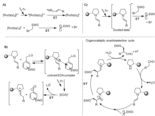
FIGURE 1. Strategies in stereoselective photocatalytic addition of bromo derivatives: A, asymmetric photocatalysis with [\text{Ru}(\text{bpy})_3]^{2+} ; B, asymmetric photocatalysis induced by EDA complex; C, enamine photo-induced electron transfer.
