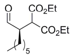
36 37 6 , 82%, 92% ee
