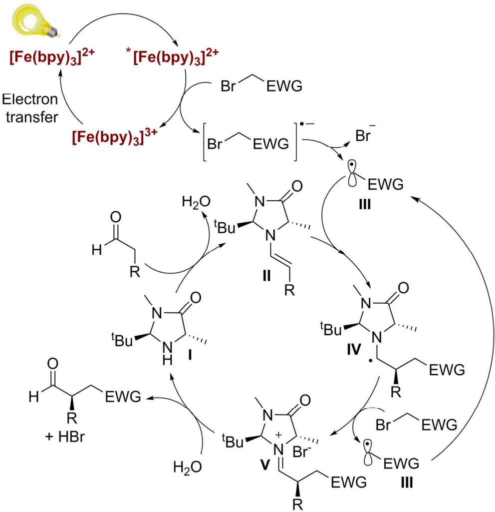
Suggested catalytic cycle for the Fe(II) alkylation. 115x120mm (300 x 300 DPI)
