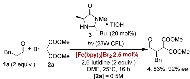
SCHEME 1. Optimized conditions for the [\text{Fe}(\text{bpy})_3]\text{Br}_2 photocatalyzed reaction.
