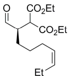
44 45 7 , 78%, 97% ee
