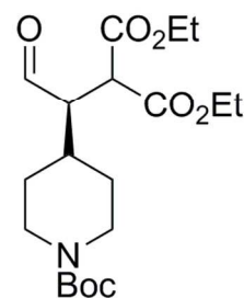
60 9 , 60%, 89% ee
