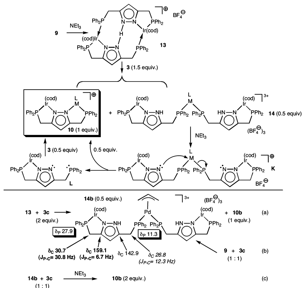
Scheme 8
