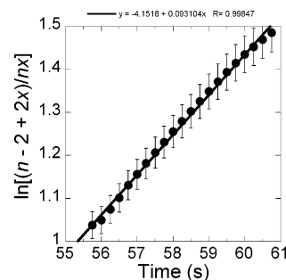
Figure 2. Kinetics of the reaction of morpholine (5.99 mM) with [(\eta^3\text{-PhC}_3\text{H}_3\text{Ph})\text{Pd}(\text{PPh}_3)_2]^+\text{BF}_4^- (C 0 = 1 mM) in DMF at 10 °C, as monitored by UV spectroscopy at 345 nm, performed in a 1 mm cell: 14 plot of \ln[(n - 2 + 2x)/nx] versus time (see eq 2).
