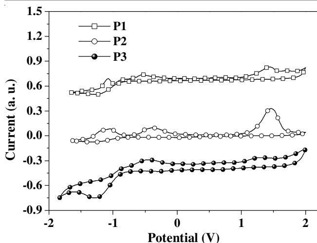
Fig. 3. Cyclic voltammograms of the copolymers at a scan rate of 100 mV/s in anhydrous acetonitrile solution with 0.1 M tetrabutyl ammonium perchlorate
