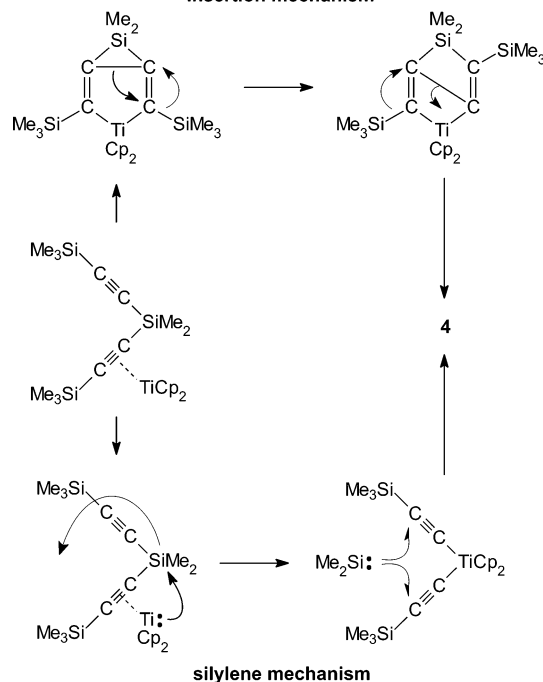
Scheme 6
