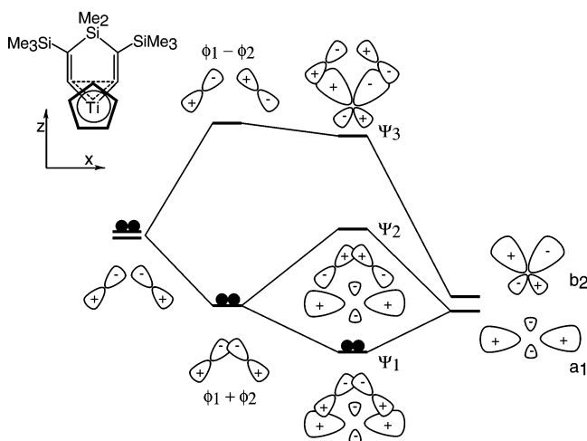
Scheme 6
