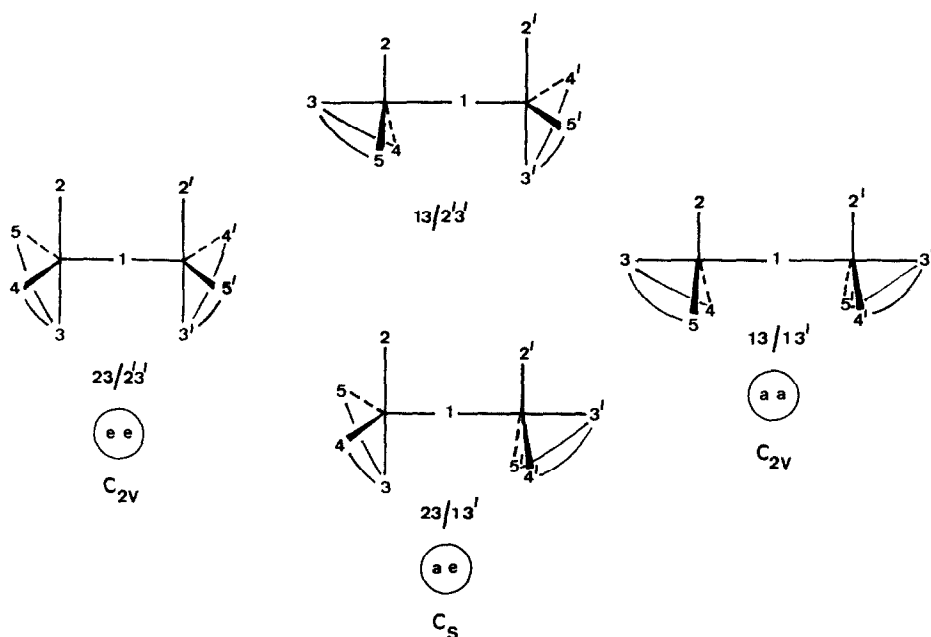
Fig. 4. The three possible isomers of 1 , their symbols and symmetry. The isomer ae can be represented by two different pairs of configurations, 13/2'3' and 23/13', while the isomers ee and aa each correspond to a single pair of configurations.
