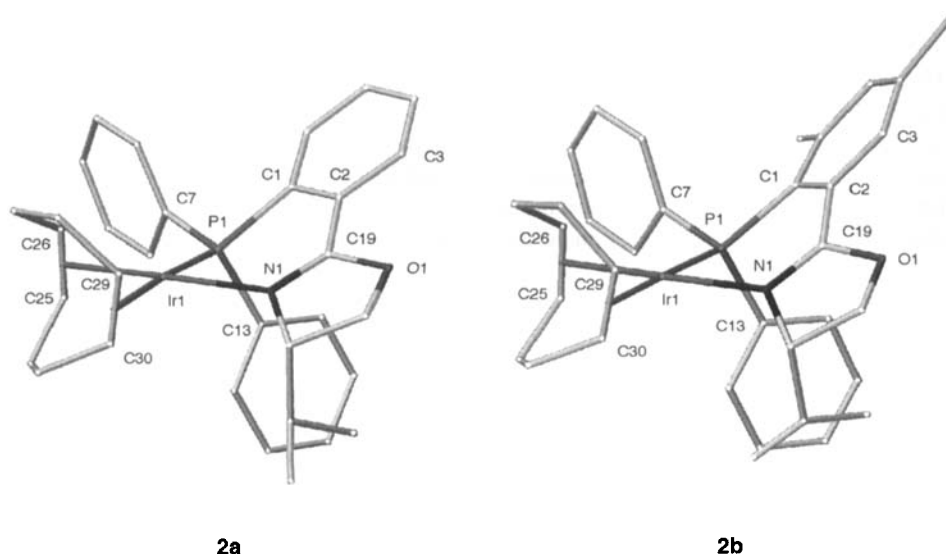
Figure 1. Crystal structures of complexes 2a and 2b . The H atoms and the PF 6 – ion are omitted for clarity.
