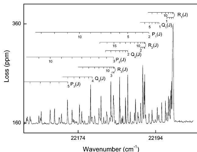
Figure 1. Cavity ring-down laser absorption spectrum of the (0,0) band of the E 3 Δ–X 3 Δ transition of VN.
