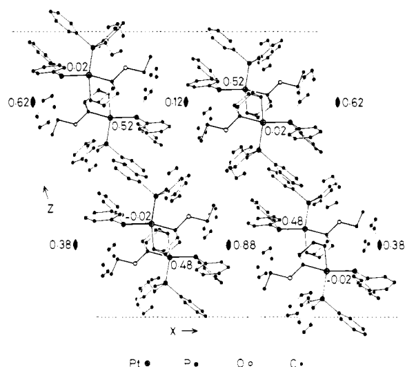
Figure 1. Pt[C 6 H 9 OC 2 H 5 ][P(C 6 H 5 ) 3 ] 2 (2). Contents of a unit cell viewed down the b axis. The outline of the unit cell is shown by broken lines. Adjacent to each platinum atom is given the y coordinate of that atom. The oxygen atoms of the water of crystallization are disordered and lie on the crystallographic twofold axes; the y coordinate adjacent to each axis is that of the midpoint of a pair of half-oxygen atoms.
