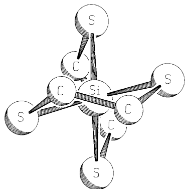
Fig. 1. SCHAKAL plot of the calculated structure of 1 (B3LYP/6-31G*), hydrogen atoms omitted for clarity, showing the partial planarization of the \text{SiS}_4 tetrahedron.
