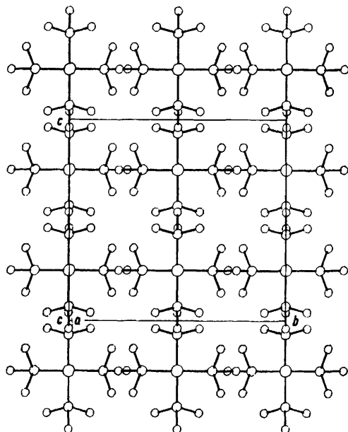
FIGURE 3 Packing diagram of [\text{Rh}(\text{PMe}_3)_4]\text{Cl}
