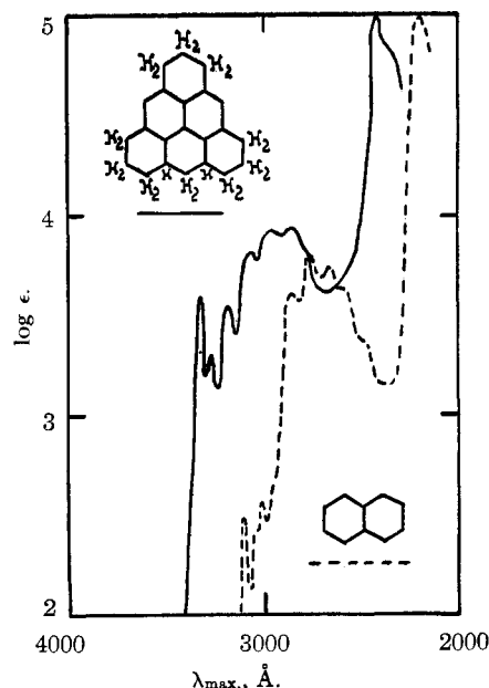
Fig. 3.—, absorption spectrum of dodecahydrotriangulene (XII) in alcohol. Maxima in Å. with log \epsilon in parentheses: 3350 (3.60), 3285 (3.29), 3180 (3.54); 3060 (3.82), 2950 (3.95), 2860 (3.93); 2420 (5.00). — — — —, absorption spectrum of naphthalene in alcohol. Maxima in Å. with log \epsilon in parentheses: 3110 (2.48), 3010 (2.56); 2850 (3.62), 2750 (3.80), 2660 (3.75), 2570 (3.64); 2210 (5.00).
