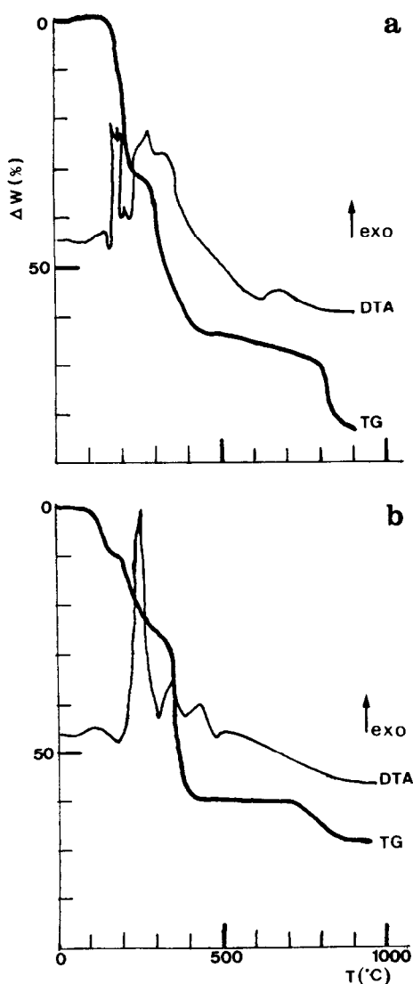
Fig. 1. Mass loss and DTA curves of [\text{MoCl}_2(\text{PMe}_3)_4] : (a) in inert atmosphere; (b) in air.
