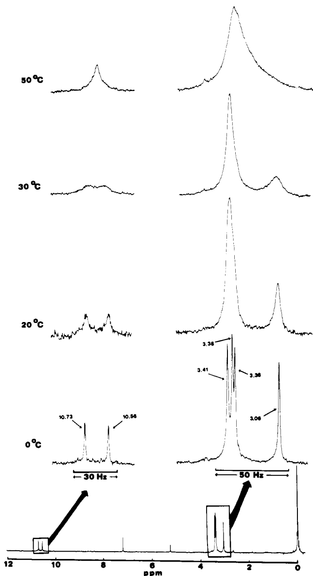
Figure 1. Representative variable-temperature ^1\text{H} NMR spectra of 2 over the range 273–323 K which illustrate averaging of the two acetylenic proton signals and the four dithiocarbamate methyl signals, respectively.
