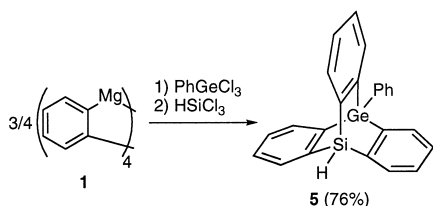
Scheme 2. Synthesis of 10-phenyl-10-germa-9-silatriptycene 5 .
