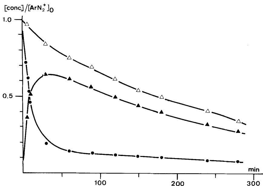
Fig. 6. Kinetics of decomposition at pH 9.70, 50.0°, [\text{CO}_3^{2-}] = 0.01 \text{ mol/l} . ● [conc.] = [\text{ArN}_2^+] , ▲ [conc.] = [\text{trans-ArN}_2\text{O}^-] , △ [conc.] = [\text{diazo}]_{\text{tot}} = [\text{ArN}_2^+] + [\text{trans-ArN}_2\text{O}^-]
