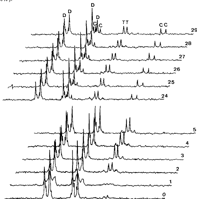
Fig.10. Part of a series of ^1H -NMR spectra used for kinetic measurements in D_2O (pD=9.7, 50^\circ , [ArN_2^+]_0 = 0.06 mol/l). D=diazonium ion, T= trans -diazotate, C=4-diazo-2,5-cyclohexadien-1-one. Spectra 0-5 and 18-23 are the first six and last six spectra, respectively, of a series of 30 taken at 90 s intervals.
