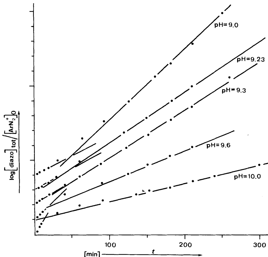
Fig. 8. Evaluation of the kinetics of decomposition at 20.0° as a function of the pH-value
