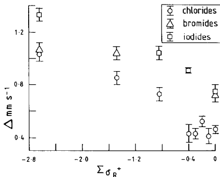
Fig. 3. Quadrupole splitting, \Delta(\text{mm s}^{-1}) vs. \Sigma Hammett resonance constant \Sigma\sigma_{\text{R}}^{+} for the \text{Fe(III)(por)X} data (por = tetraphenyl substituted porphyrins) presented in Table I.
