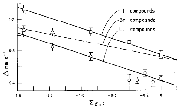
Fig. 2. Quadrupole splitting, \Delta(\text{mm s}^{-1}) vs. \Sigma Hammett mesomeric constant \Sigma\sigma_{\text{R}}^{\circ} for the \text{Fe(III)(por)X} data (por = tetraphenyl substituted porphyrins) presented in Table I.
